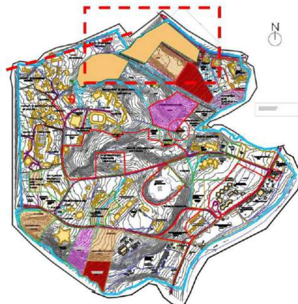
MASTER PLAN OF TU KIRTIPUR, KATHMANDU
